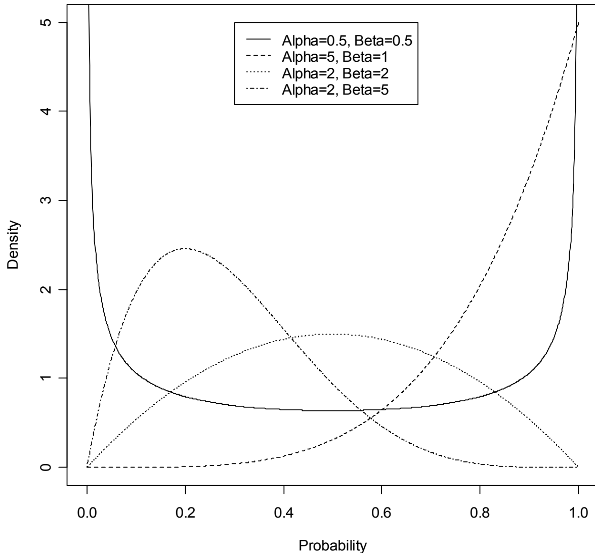
Figure 4. Beta Distributions
